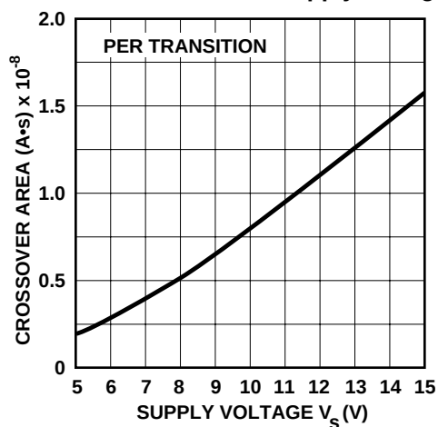
Crossover Area vs. Supply Voltage
