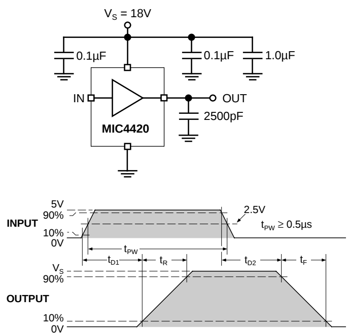
Figure 1b. Noninverting Driver Switching Time
