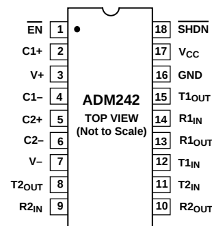
Figure 11. ADM242 DIP/SOIC Pin Configuration
