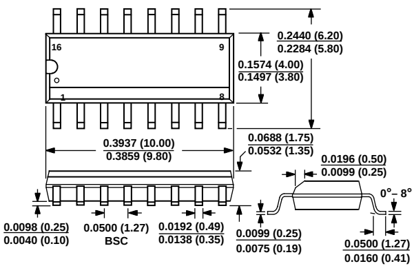
16-Lead Narrow SOIC (R-16N)
