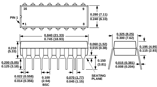
16-Pin Plastic DIP (N-16)
