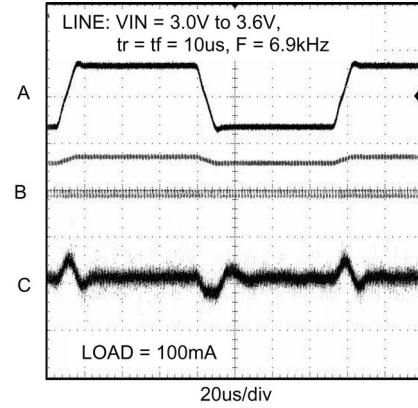
Line Transient Response (PWM Mode)
