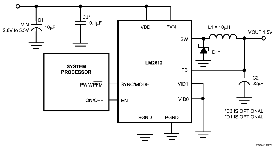
FIGURE 1. Typical Operating Circuit
