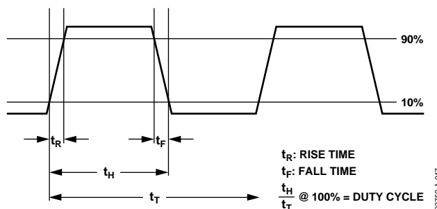
Figure 18. Duty Cycle of External Clock
