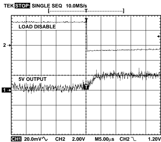
Figure 13. 5V Output Transient Response, Load Disconnected
