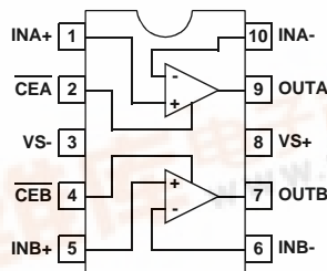
EL5292A (10-PIN MSOP) TOP VIEW
