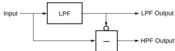
Figure 12. Complementary Bandsplit Filter
