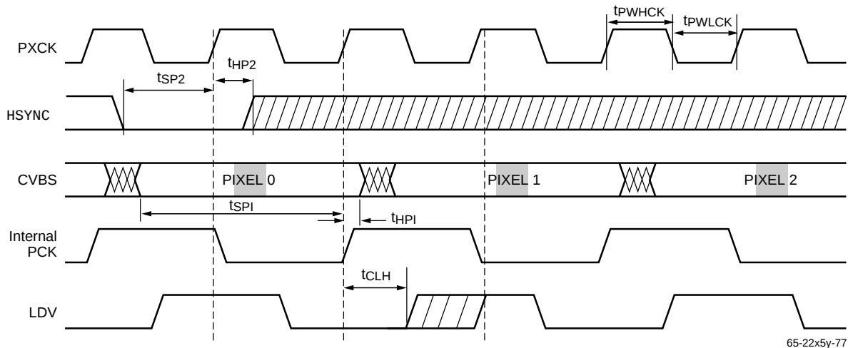
Figure 41. Input Timing Parameters
