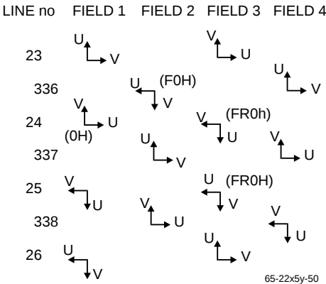
Figure 9. Chrominance Vector Rotation Over 4 Fields in PAL
