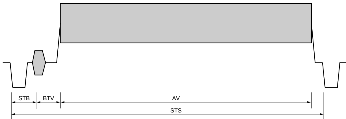
Figure 27. Horizontal Timing
