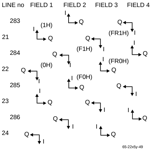
Figure 8. Chrominance Vector Rotation Over 4 Fields in NTSC
