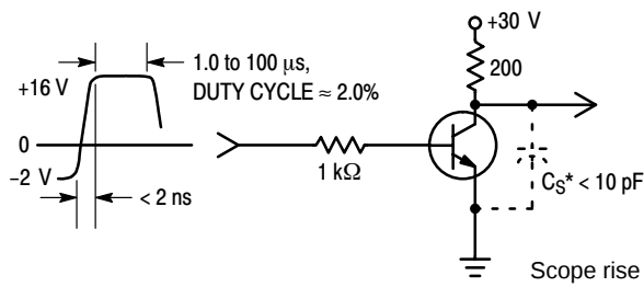
Figure 1. Turn-On Time
