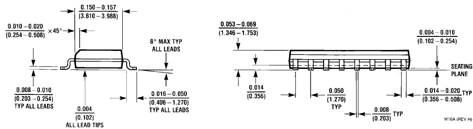
16-Lead Molded Small Outline Package (M)
