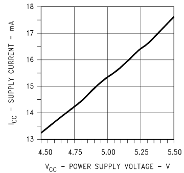
Disabled Supply Current vs Power Supply Voltage
