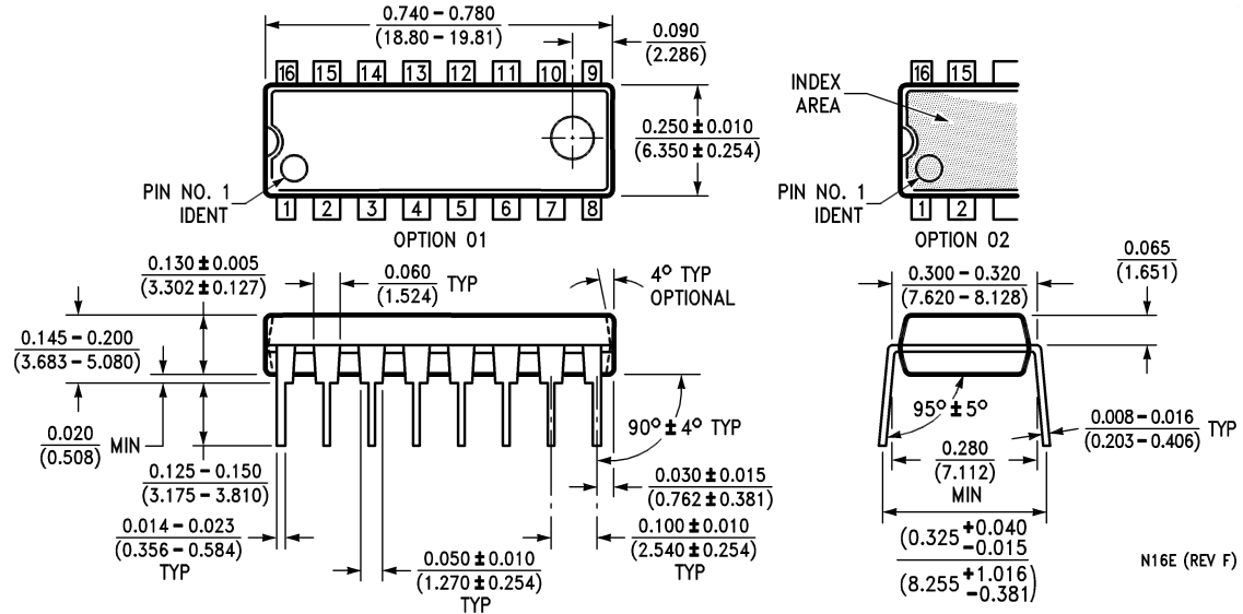
16-Lead Molded Dual-In-Line Package (N)
