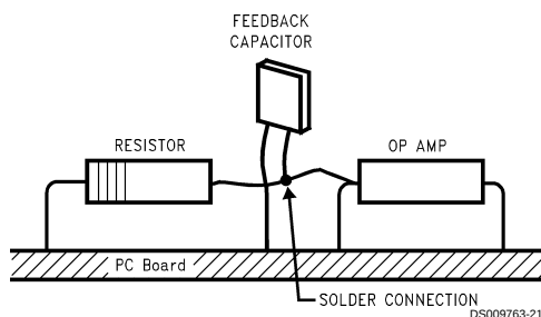
FIGURE 10. Air Wiring
