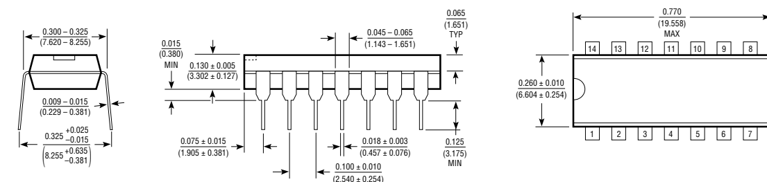
N Package 14-Lead Plastic DIP
