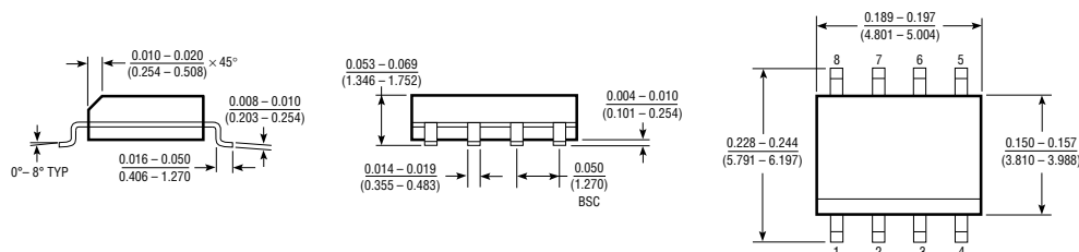
S8 Package 8-Lead Plastic SOIC
