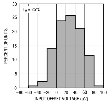
Distribution of Offset Voltage at V_S = \pm 1.0V (In All Packages)
