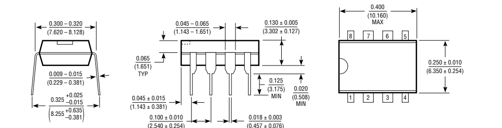
N8 Package 8-Lead Plastic DIP
