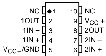
TLV2252M, TLV2252AM ... U PACKAGE (TOP VIEW)
