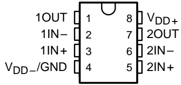
TLV2252M, TLV2252AM ... JG PACKAGE (TOP VIEW)
