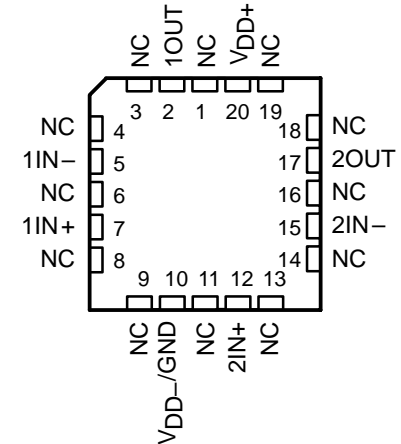
TLV2252M, TLV2252AM ... FK PACKAGE (TOP VIEW)
