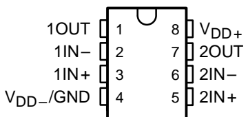
TLV2252M, TLV2252AM ... U PACKAGE (TOP VIEW)
