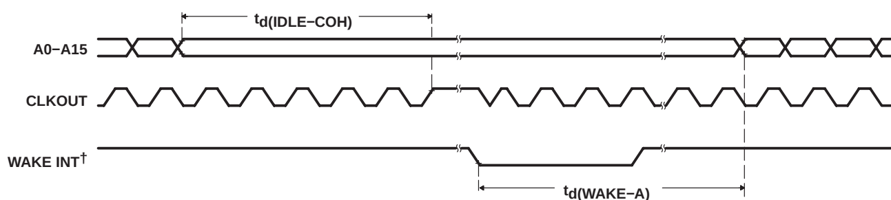
Figure 31. IDLE2 Entry and Exit Timing – LPM1
