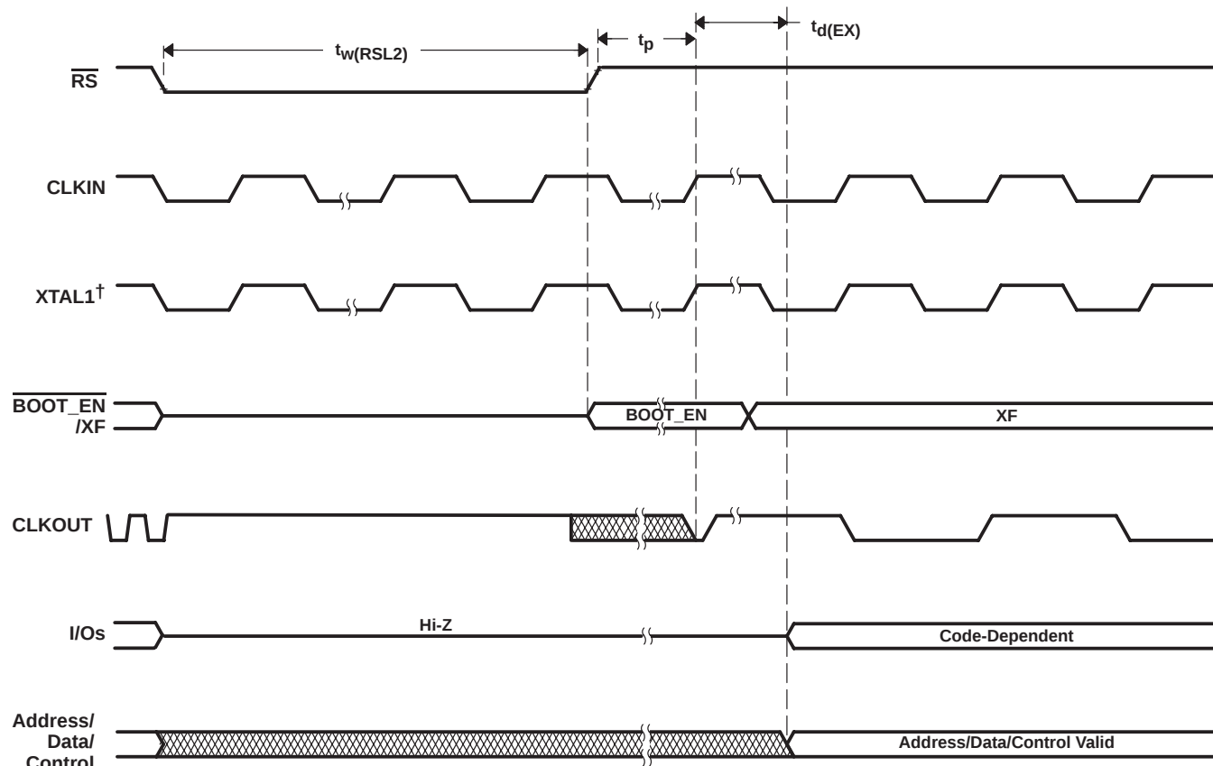
Figure 28. Warm Reset
