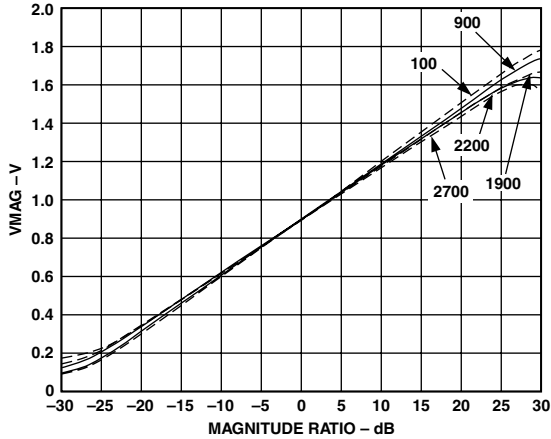
TPC 1. Magnitude Output (VMAG) vs. Input Level Ratio (Gain) V_{INPA}/V_{INPB} , Frequencies 100 MHz, 900 MHz, 1900 MHz, 2200 MHz, 2700 MHz, 25°C, P_{INPB} = -30\text{ dBm} , (Re: 50\ \Omega )
