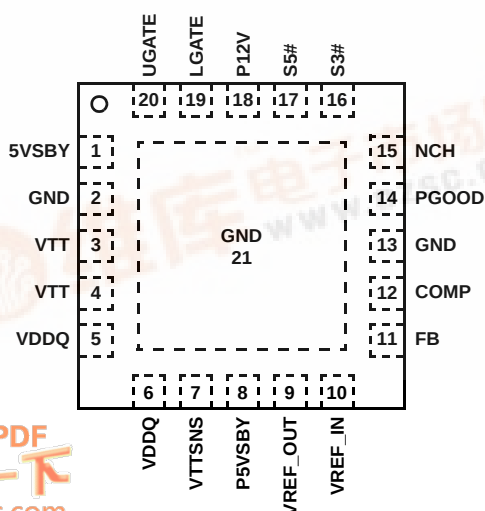
ISL6532 (QFN) TOP VIEW
