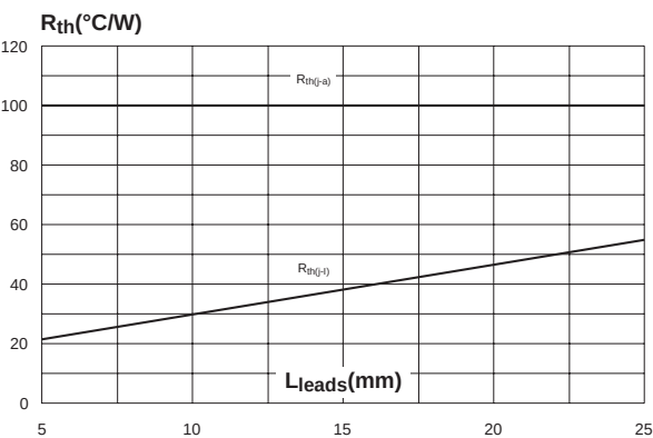
Fig. 10: Thermal resistance versus lead length (DO-41).
