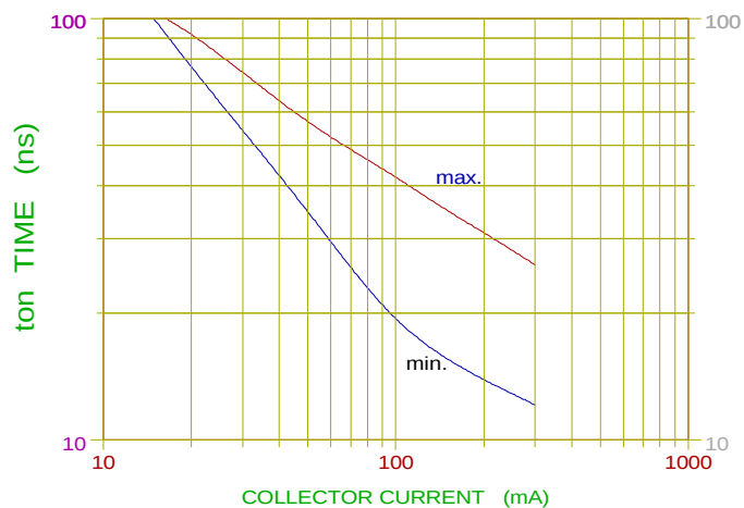
SWITCHING TURN - ON TIME T_J = 25^\circ\text{C} I_C/I_B = 10
