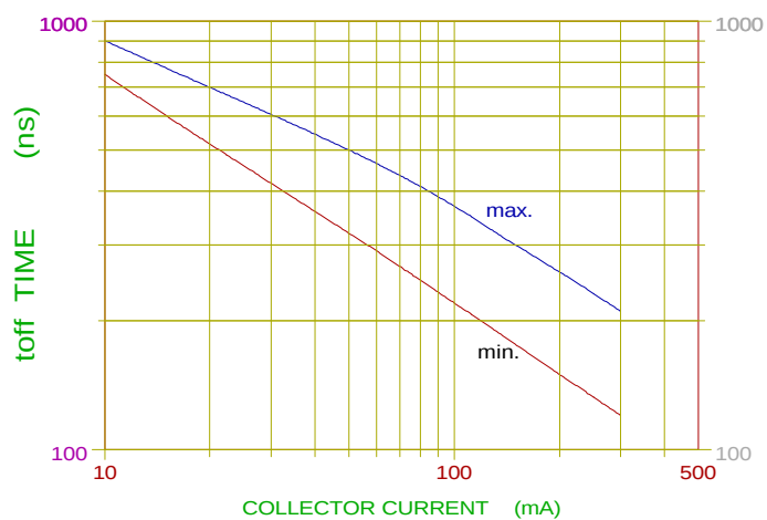
SWITCHING TURN - OFF TIME T_J = 25^\circ\text{C} I_C/I_B = 10
