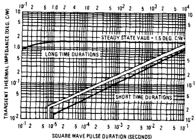
Fig. 15 — Maximum Transient Thermal Resistance Vs. Square Wave Pulse Duration (Rectangular Current Waveform), 2N5204 Series
