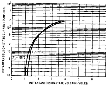
Fig. 14 — Maximum Instantaneous On-State Voltage Vs. Instantaneous On-State Current (Rectangular Current Waveform), 2N5204 Series
