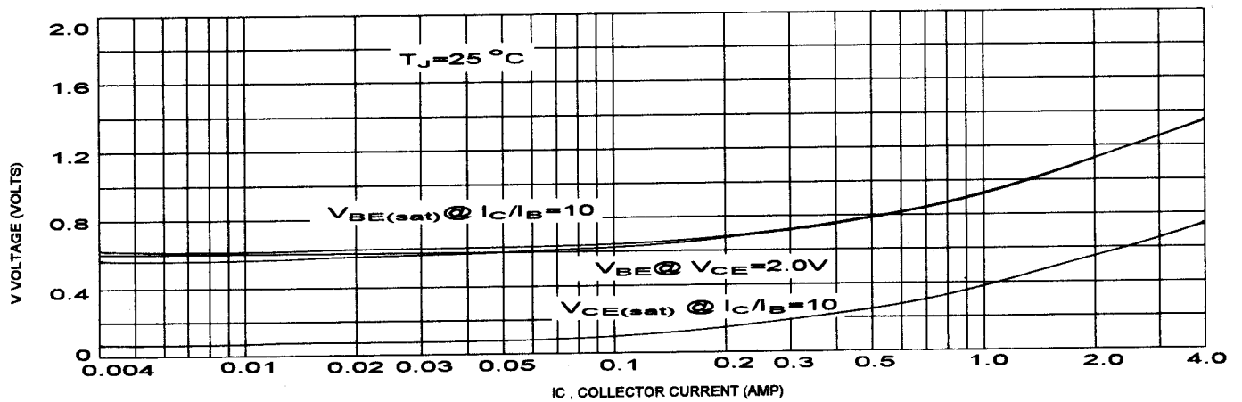
"ON" VOLTAGES
