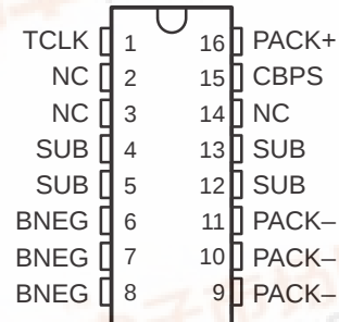
DP PACKAGE (TOP VIEW)
