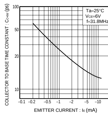
Fig.9 Collector to base time constant vs. emitter current
