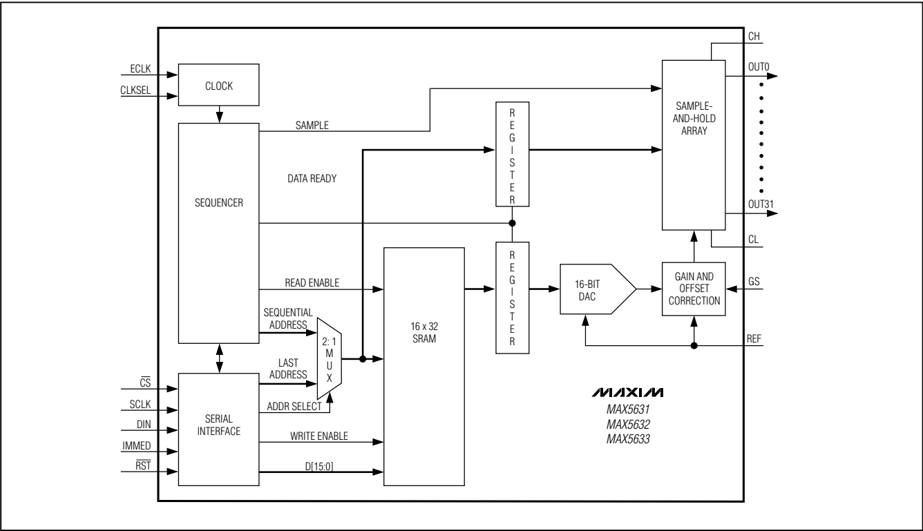
Figure 1. Functional Diagram
