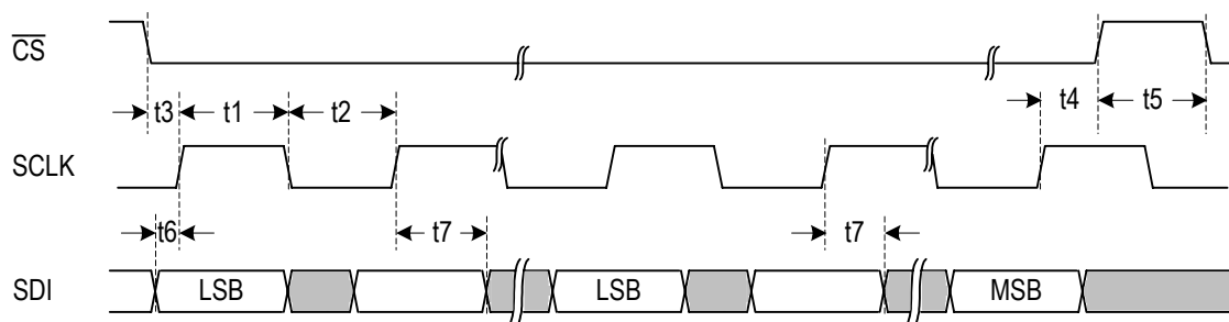
Figure-26 Serial Interface Write Timing
