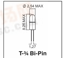
T-3/4 Bi-Pin
