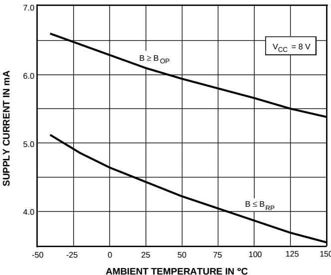
SUPPLY CURRENT
