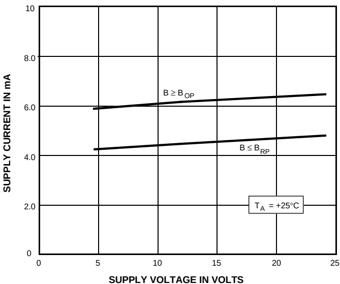
SUPPLY CURRENT
