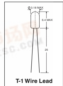
T-3/4 Bi-Pin
