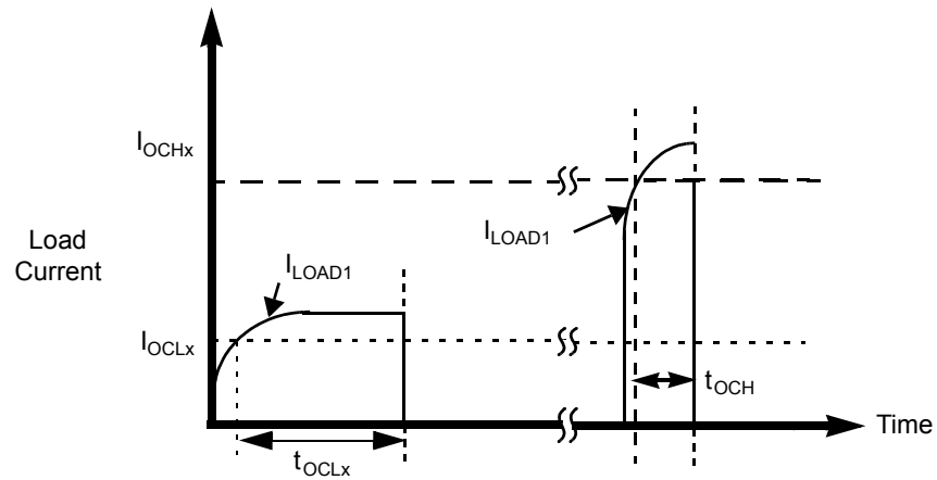
Figure 3. Overcurrent Shutdown
