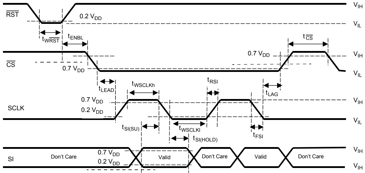
Figure 5. Input Timing Switching Characteristics
