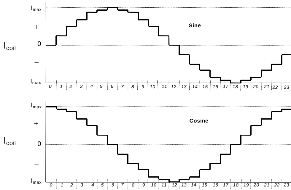
Figure 6.1 Microstepping
