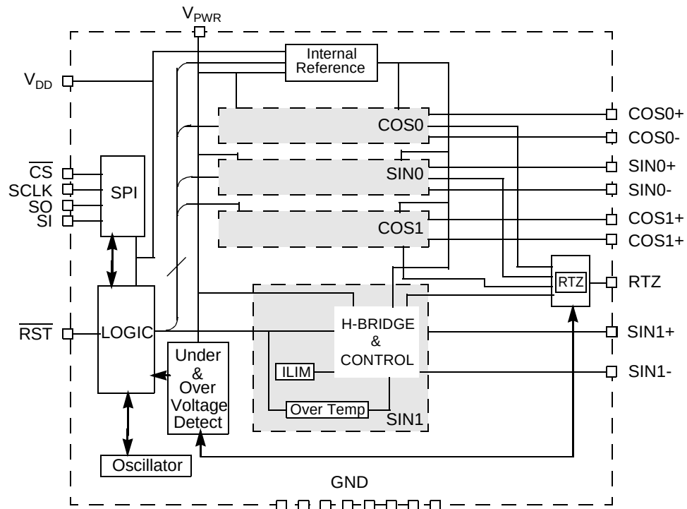
Figure 1. 33991 Block Diagram
