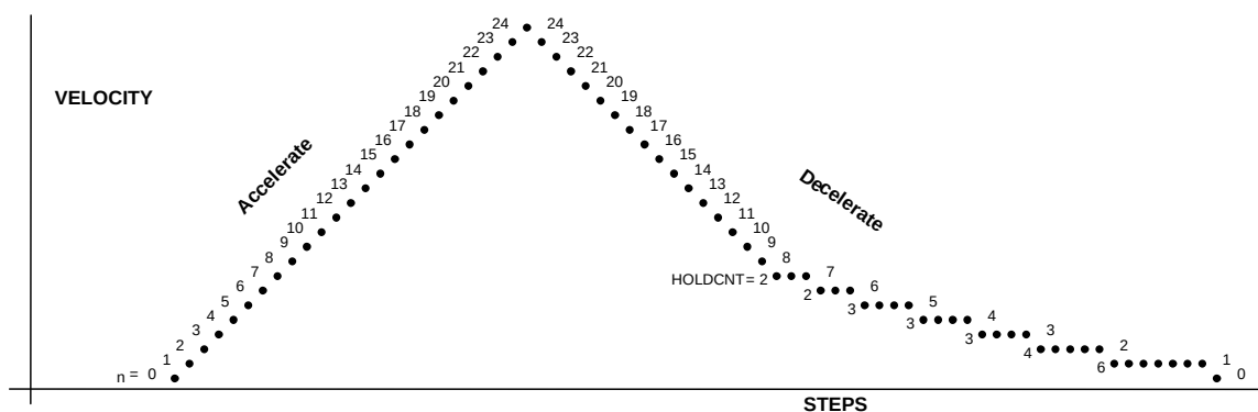
Figure 8. Deceleration Waveshaping
