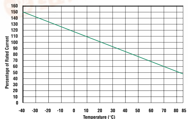
Derating Curve for 3425L Series
