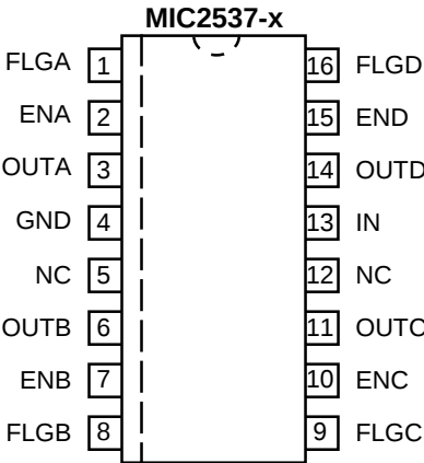
16-Lead SOP (M)
