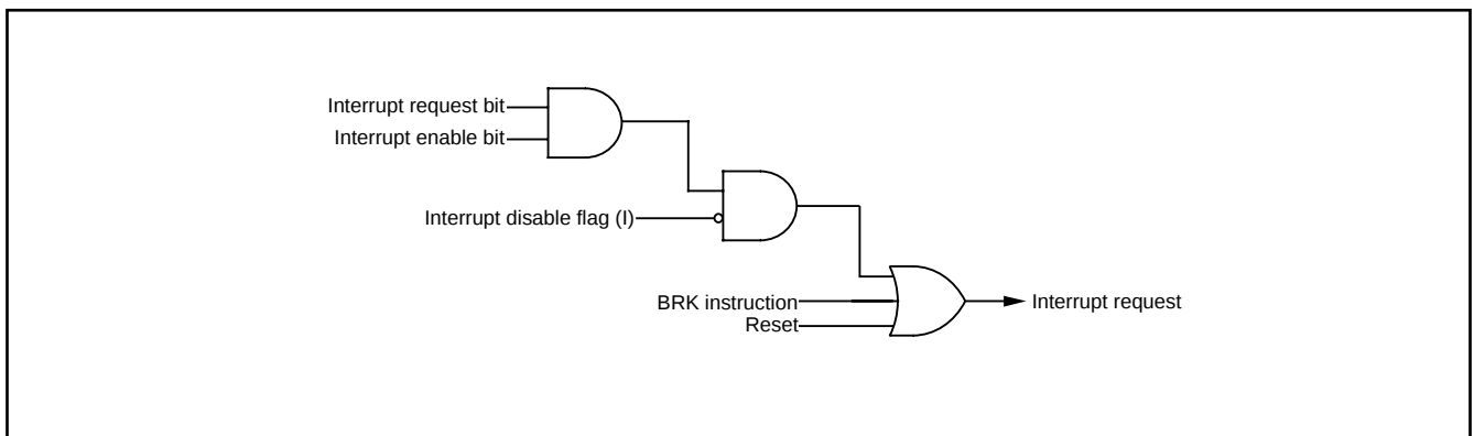
Fig. 8 Interrupt control
