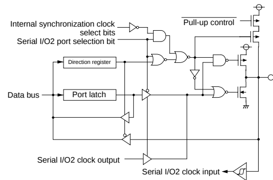
(12) Port P52
