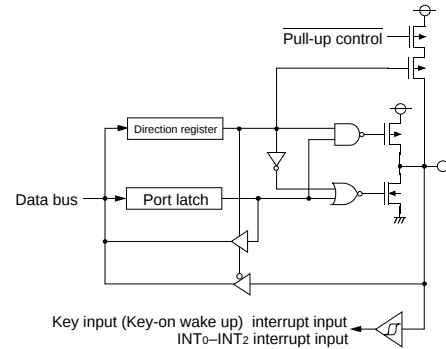
(2) Ports P2,P42,P43,P57
