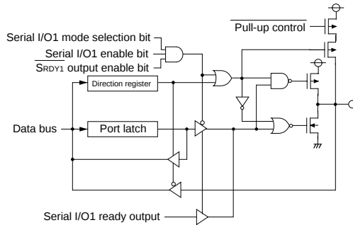
(11) Port P51
