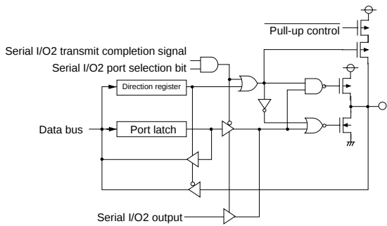
(11) Port P51
