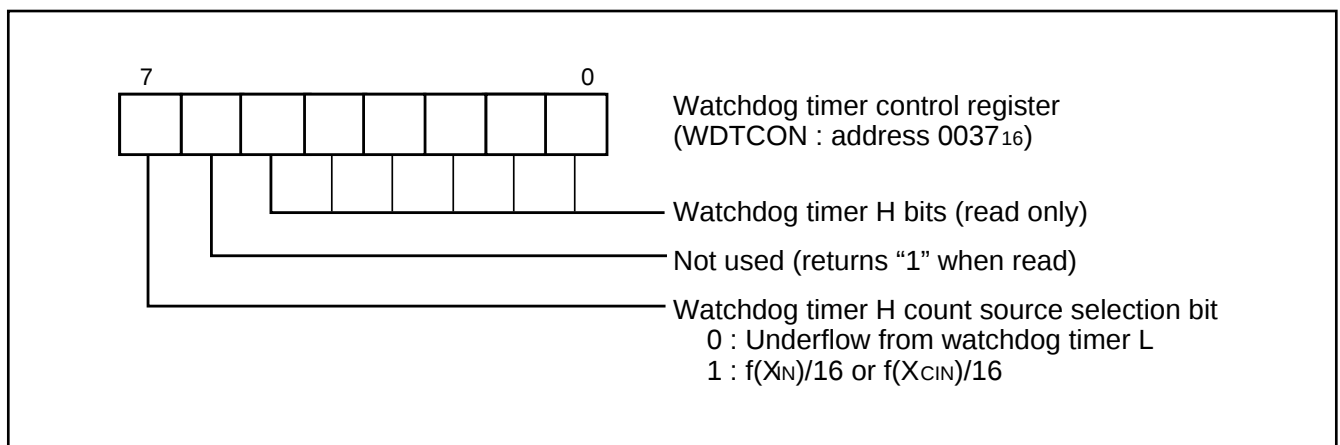
Fig. 30 Structure of watchdog timer control register
