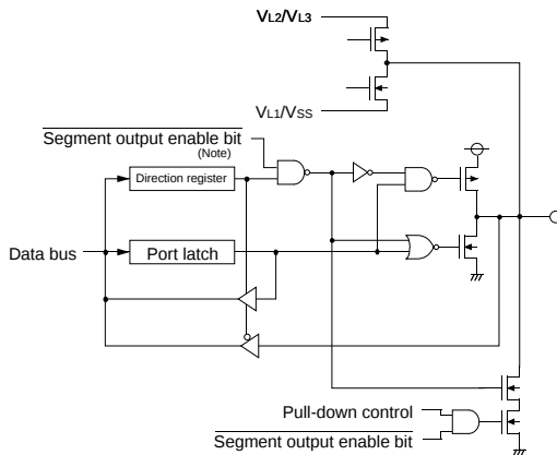
(1) Ports P0,P1
