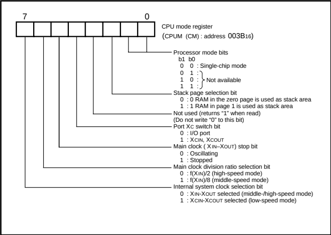
Fig. 1 Structure of CPU mode register
