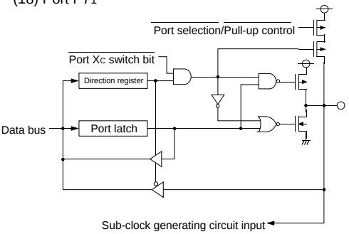
(18) Port P71
