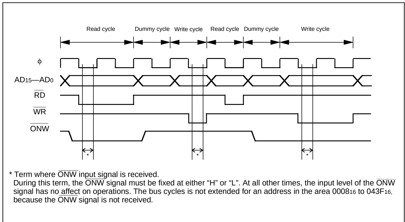
Fig. 64 \overline{\text{ONW}} function timing
