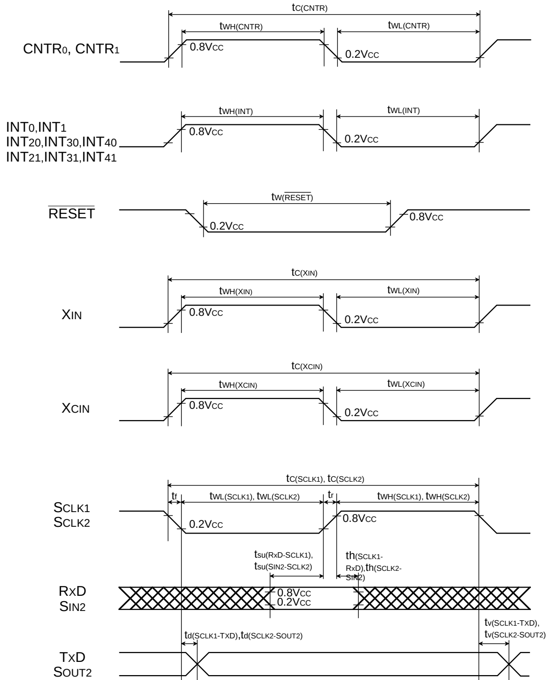
Timing diagram in single-chip mode
