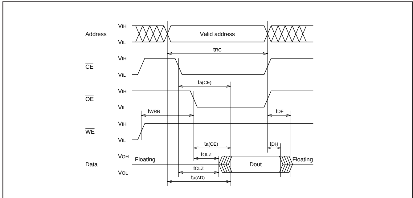
Fig. 67 Read timing
