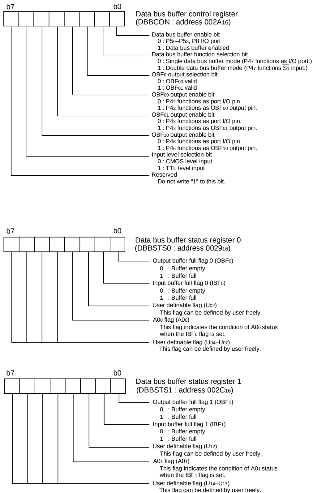
Fig. 33 Structure of bus interface related register
