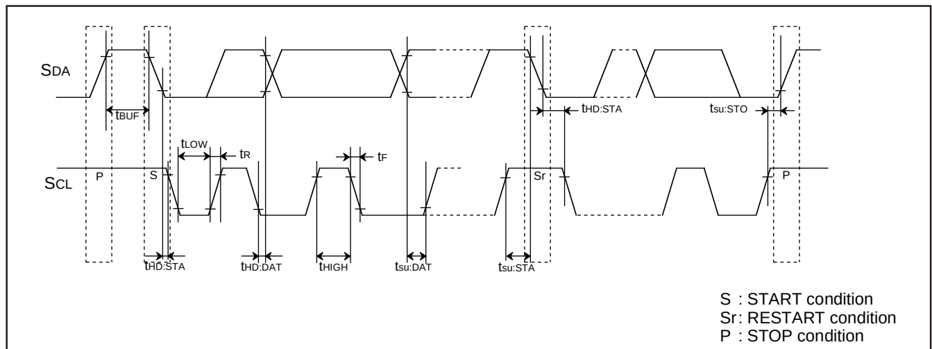
Fig. 89 Timing diagram of multi-master I 2 C-BUS
