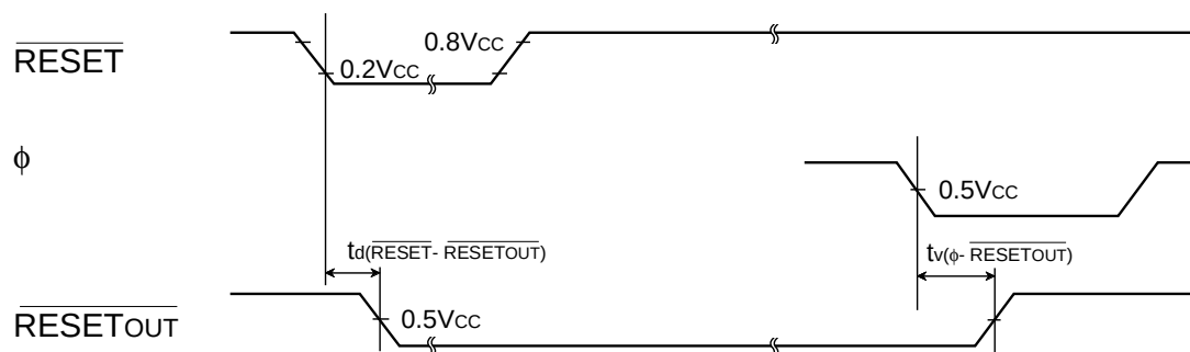
Timing diagram in microprocessor mode
