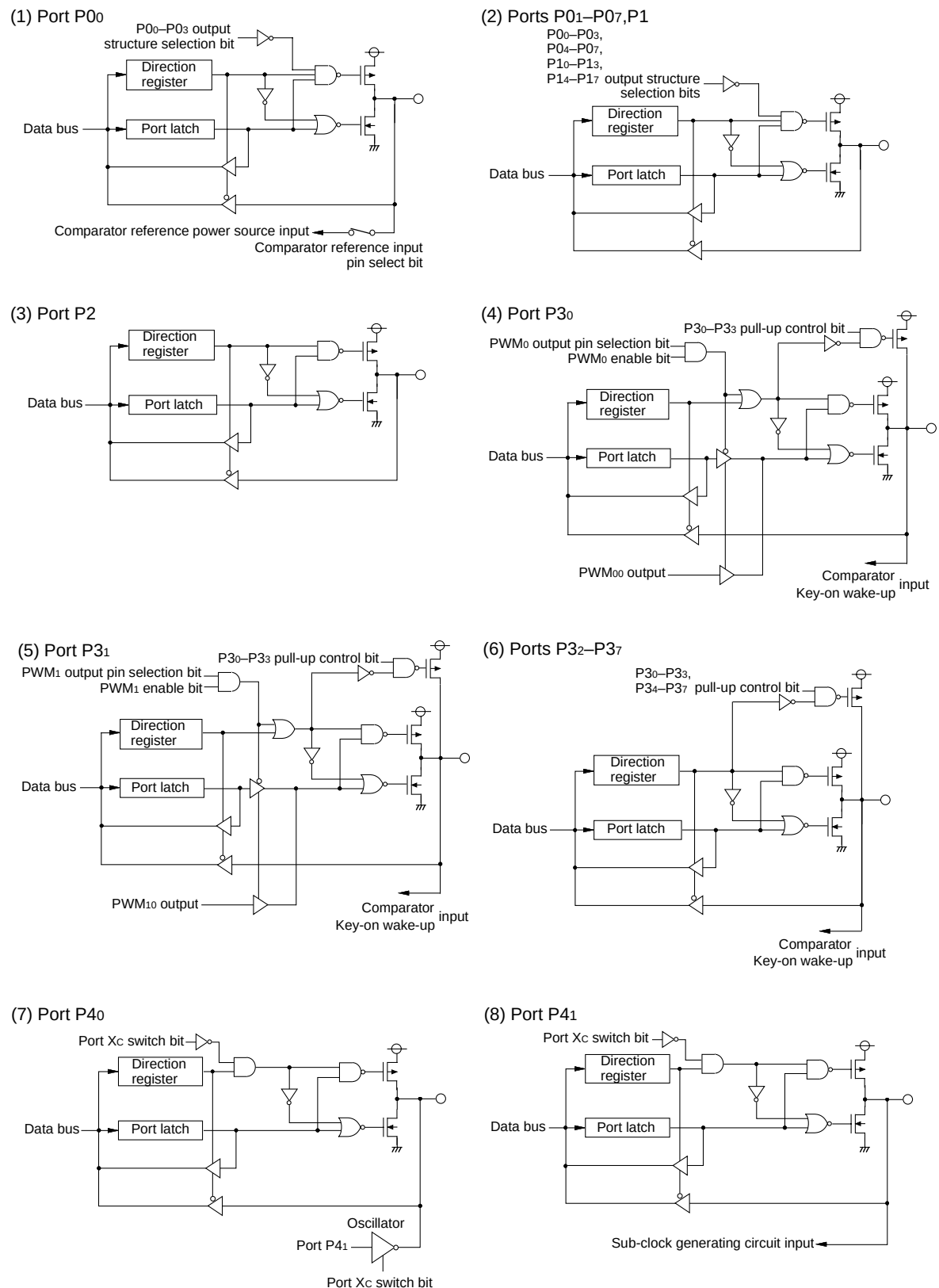
Fig. 10 Port block diagram (1)
