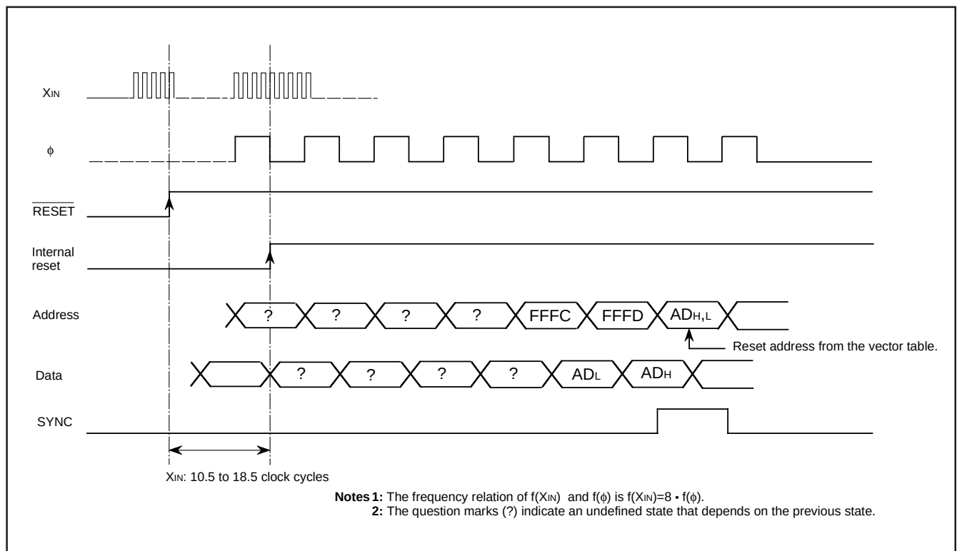
Fig. 56 Reset sequence
