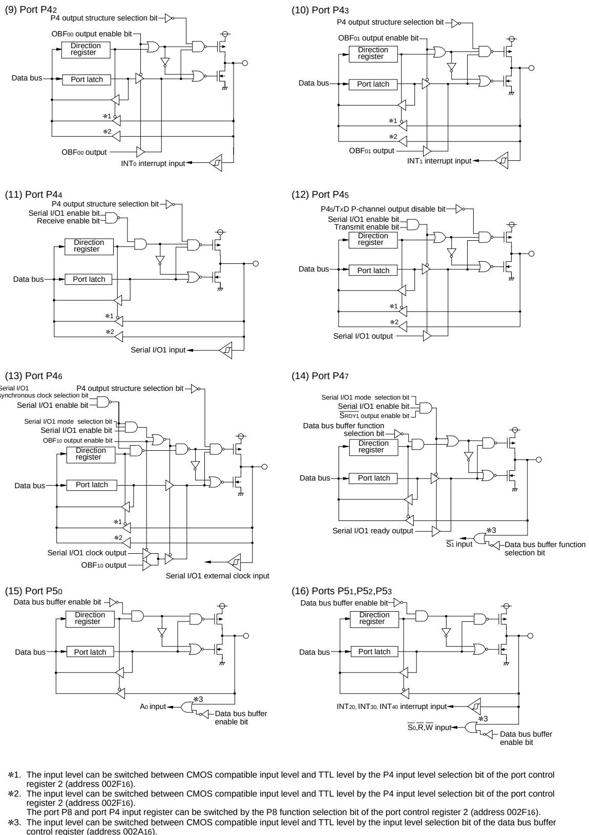
Fig. 11 Port block diagram (2)
