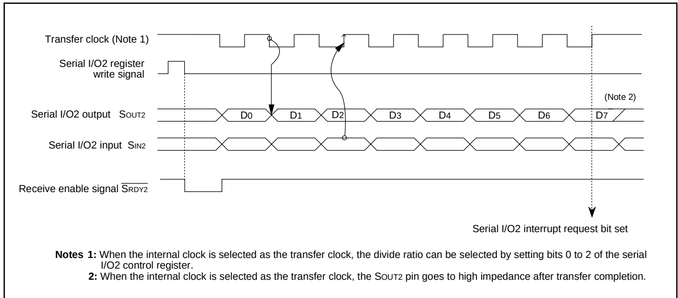
Fig. 28 Timing of serial I/O2 function
