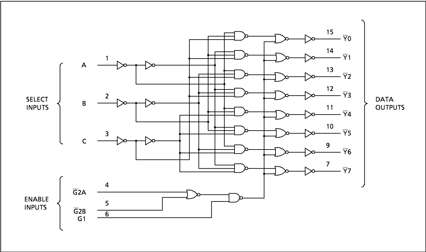
LOGIC DIAGRAM
