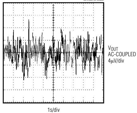
0.1Hz TO 10Hz OUTPUT NOISE ( V_{OUT} = 10V )
