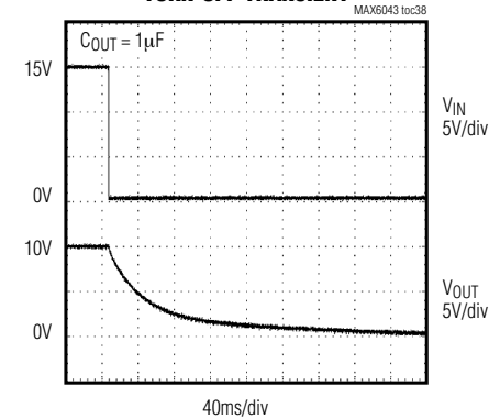
TURN-OFF TRANSIENT
