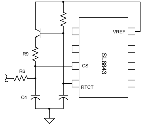
FIGURE 6. SLOPE COMPENSATION
