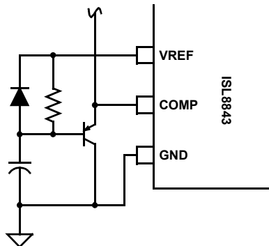
FIGURE 5. SOFT-START
