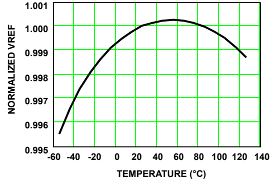
FIGURE 2. REFERENCE VOLTAGE vs TEMPERATURE
