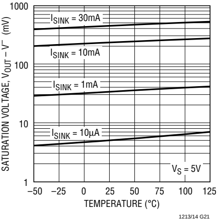
Negative Output Saturation Voltage vs Temperature
