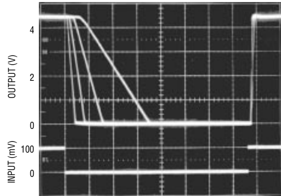
LT1213 Comparator Response (-) 20mV, 10mV, 5mV, 2mV Overdrives
