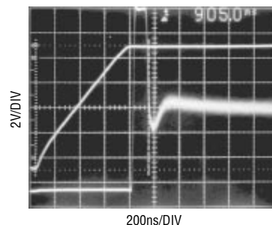
\pm 15V Settling
