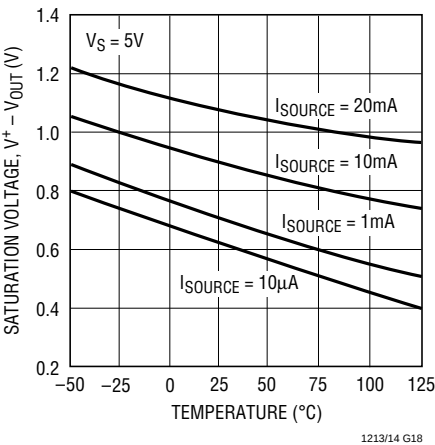
Positive Output Saturation Voltage vs Temperature
