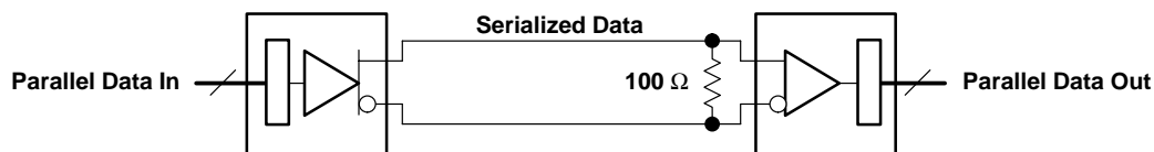
Figure 20. Single-Terminated Point-to-Point Connection
