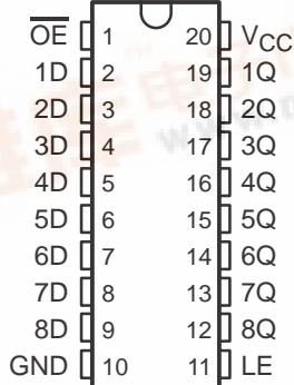
SN54HC573A ... J OR W PACKAGE SN74HC573A ... DB, DW, N, OR PW PACKAGE (TOP VIEW)
