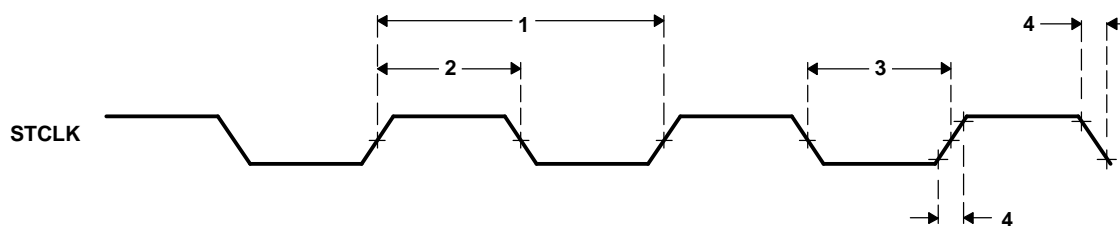
Figure 5-56. STCLK Timing
