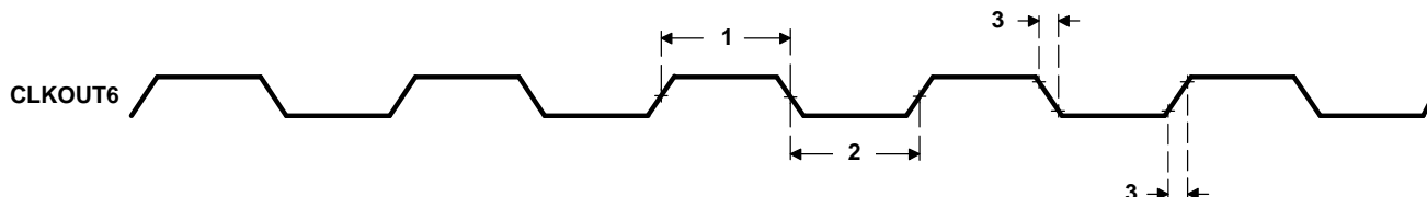
Figure 5-13. CLKOUT6 Timing
