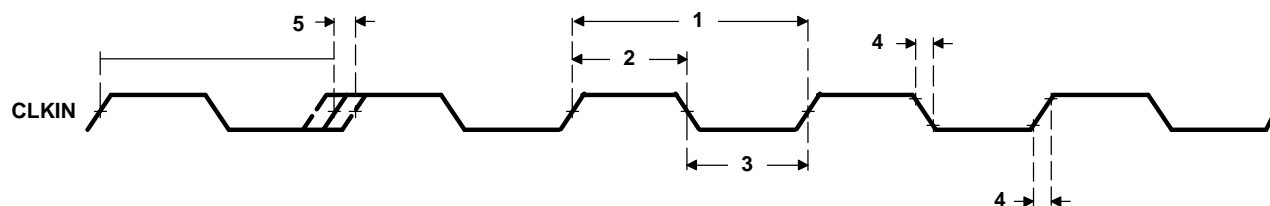
Figure 5-11. CLKIN Timing
