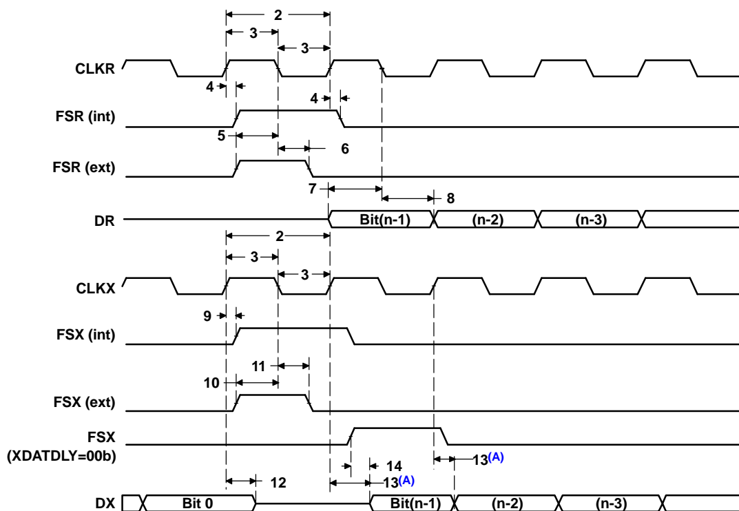
Figure 5-46. McBSP Timing
