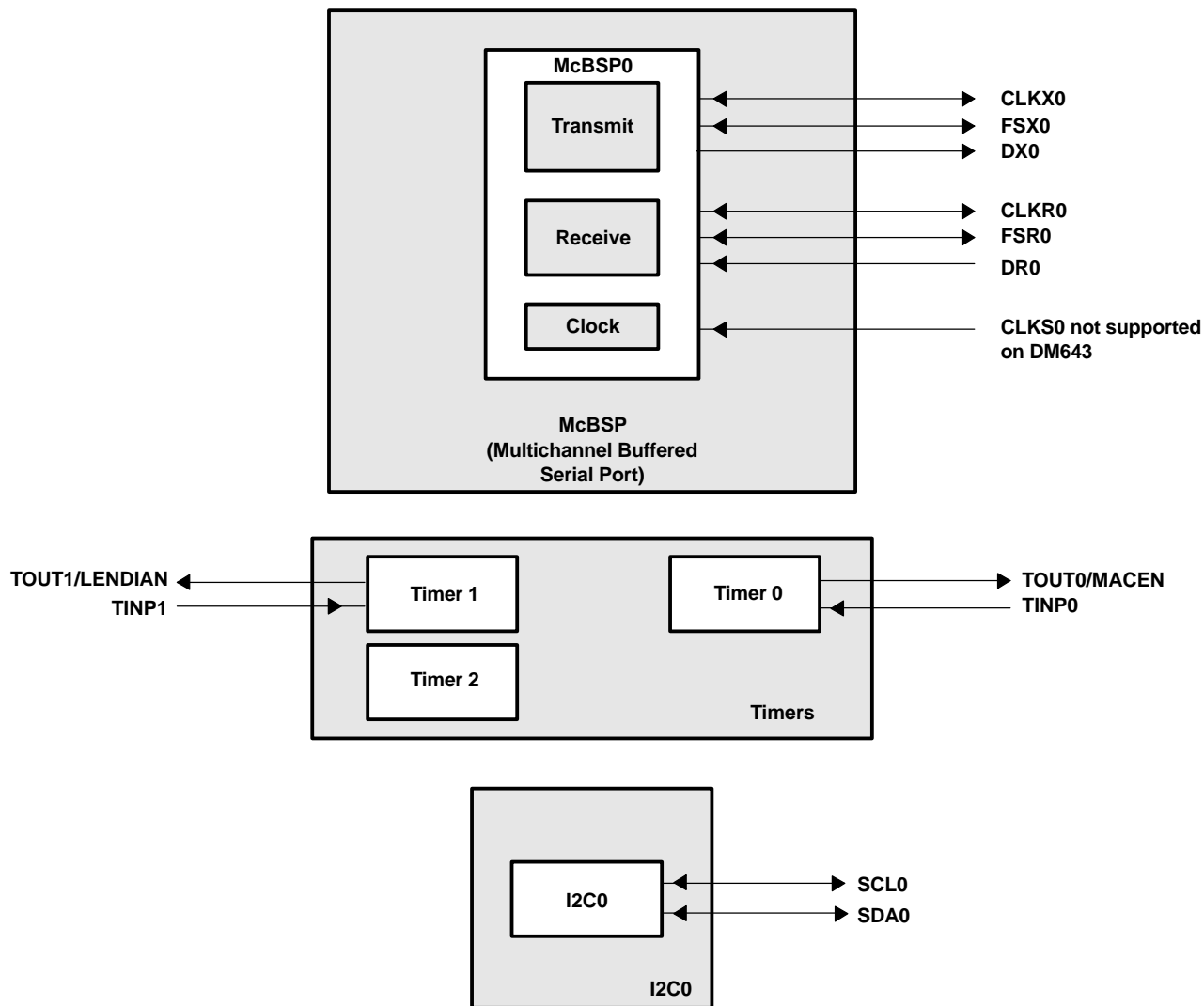
Figure 2-10. McBSP/Timer/I2C0 Peripheral Signals
