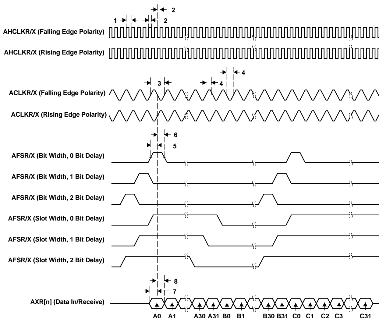
Figure 5-33. McASP Input Timings
