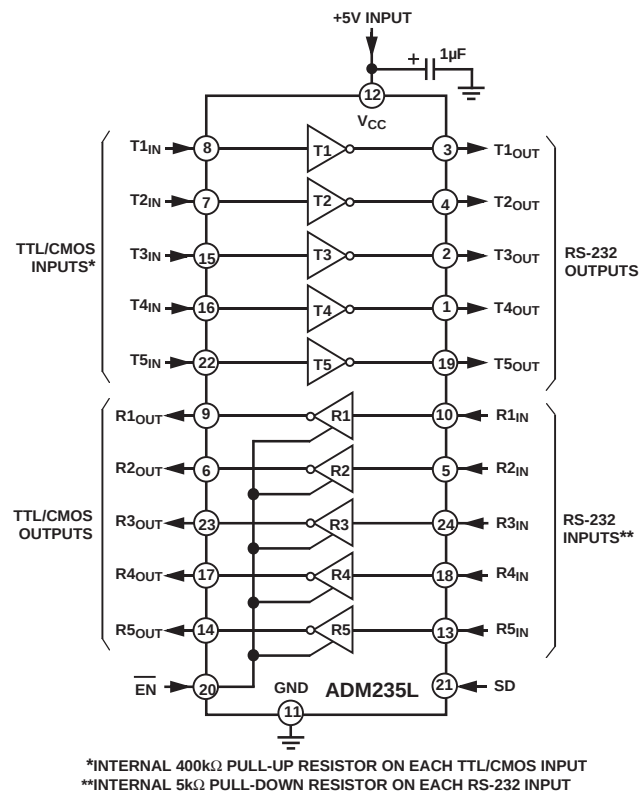
Figure 12. ADM235L Typical Operating Circuit
