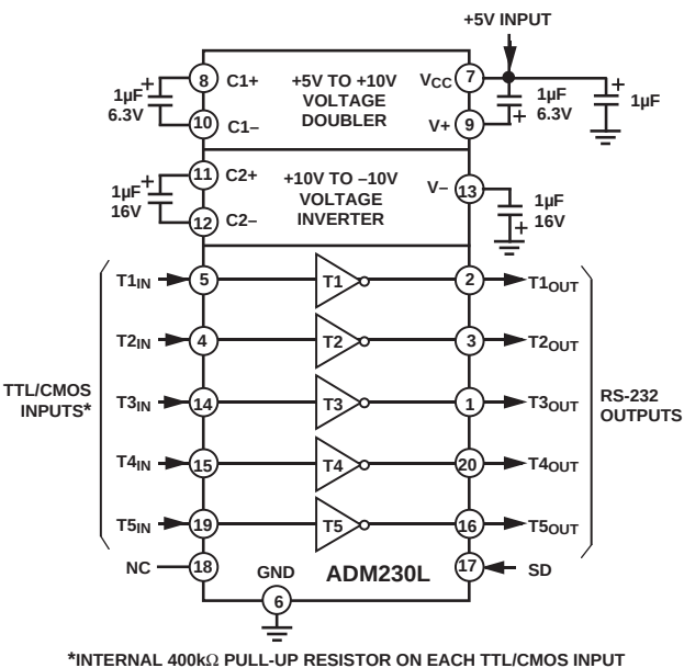
Figure 2. ADM230L Typical Operating Circuit
