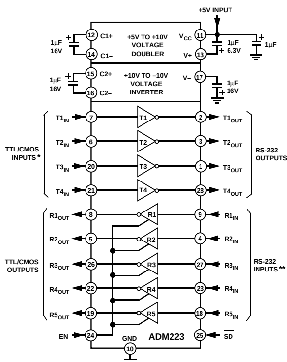
Figure 24. ADM223 Typical Operating Circuit
