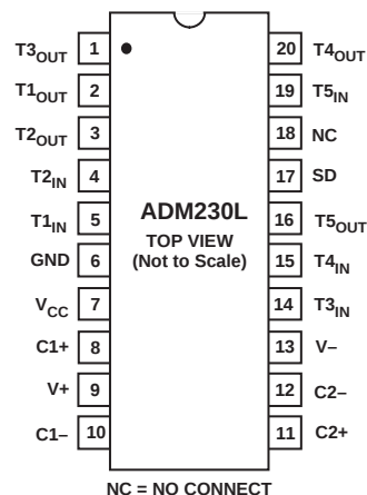
Figure 1. ADM230L DIP/SOIC Pin Configuration
