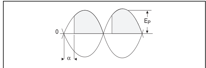
Full-wave Bridge – Waveform
