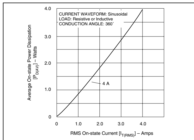
Figure E2.19 Power Dissipation (Typical) versus RMS On-state Current (4 A)
