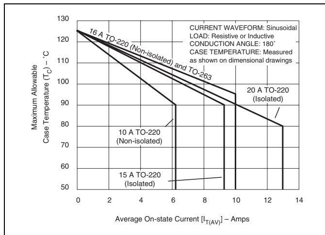
Figure E6.13 Maximum Allowable Case Temperature versus Average On-state Current (10 A through 20 A)
