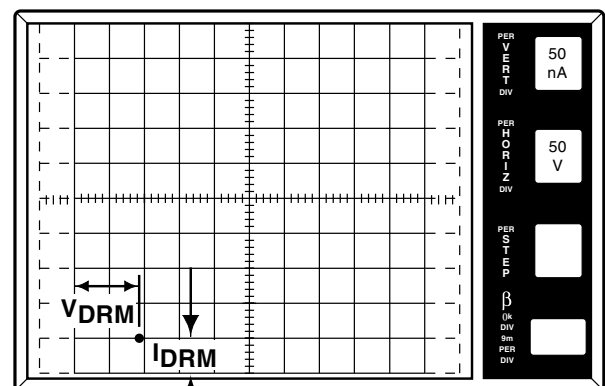
Figure AN1006.22 I_{DRM} = 50 nA at V_{DRM} = 90 V
