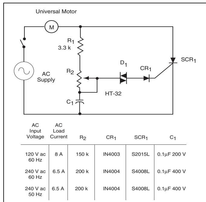
Figure AN1003.18 Half-wave Motor Control
