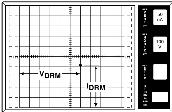
Figure AN1006.11 (+)I_{\text{DRM}} = 205 \text{ nA} at (+)V_{\text{DRM}} = 600 \text{ V}
