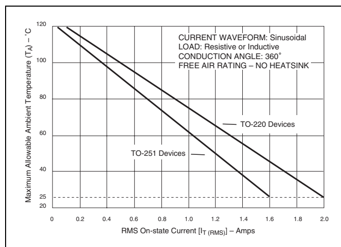
Figure E4.16 Maximum Allowable Ambient Temperature versus On-state Current
