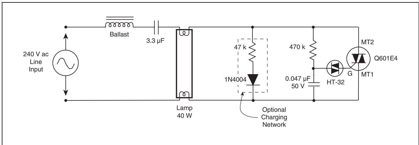
Figure AN1010.4 240 V ac Triac/Diac Circuit
