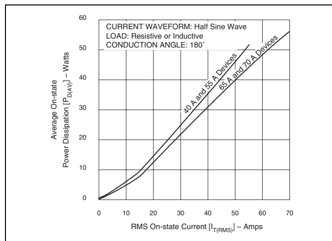
Figure E6.27 Power Dissipation (Typical) versus RMS On-state Current (40 A through 70 A)
