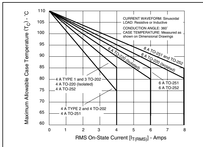
Figure E1.3 Maximum Allowable Case Temperature versus On-state Current (4 A, 6 A, and 8 A)
