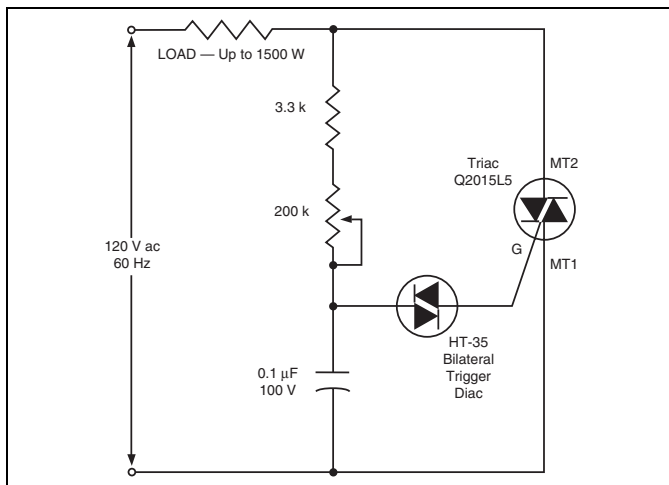
Figure E8.1 Typical Diac/Triac Full-wave Phase Control Circuit Using Lower Voltage Diacs.
