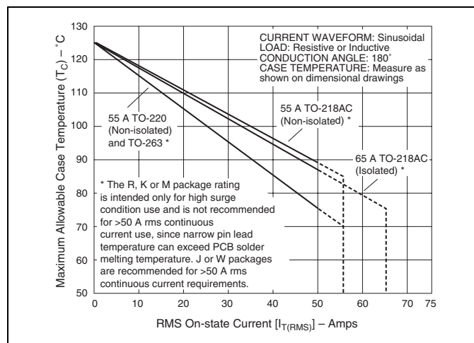
Figure E6.10 Maximum Allowable Case Temperature versus RMS On-state Current (55 A and 65 A)
