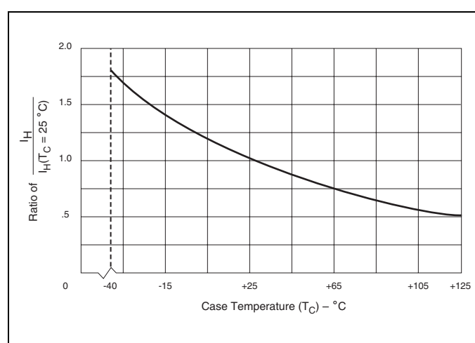
Figure E9.2 Normalized DC Holding Current versus Case/Lead Temperature
