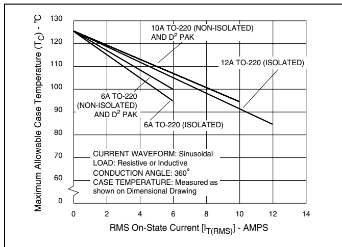
Figure E4.1 Maximum Allowable Case Temperature versus On-state Current (6 A to 12 A)
