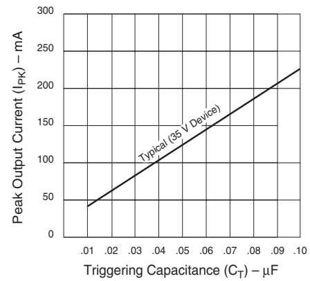
Figure E8.6 Peak Output Current versus Triggering Capacitance (Per Figure E8.5 with R_L of 20 \Omega )
