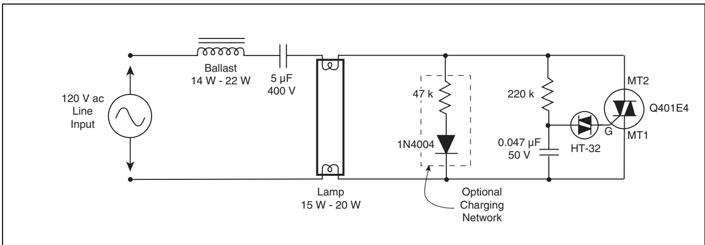
Figure AN1010.2 120 V ac Triac/Diac Circuit
