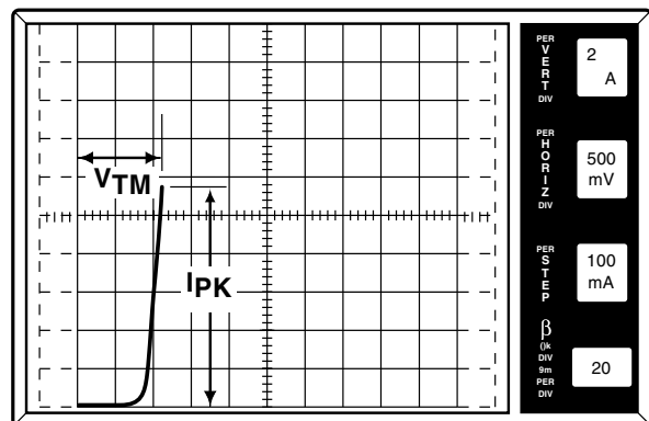
Figure AN1006.12 V_{TM (forward)} = 1.1 \text{ V} at I_{PK} = 11.3 \text{ A} (8 A rms)
