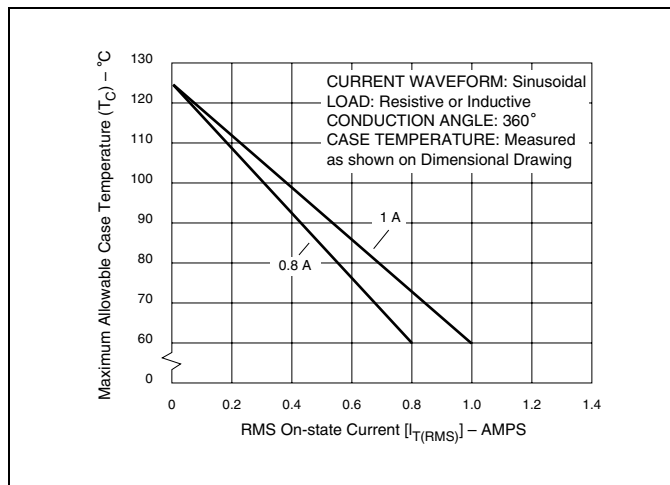
Figure E2.1 Maximum Allowable Case Temperature versus On-state Current (0.8 A and 1 A)
