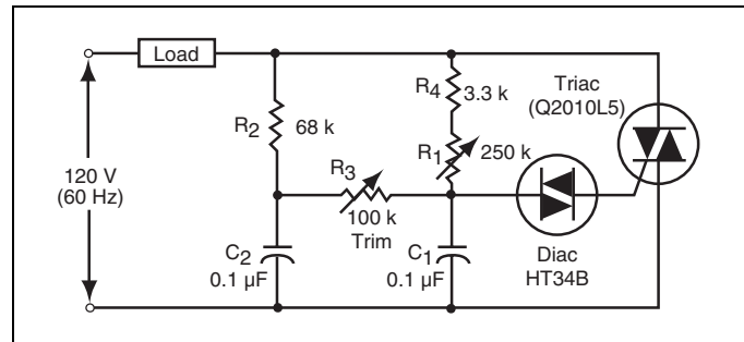
Figure AN1003.11 Extended Range Full-wave Phase Control
