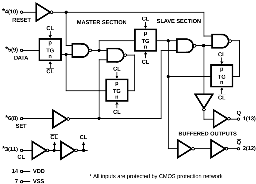
FIGURE 1. ONE OF TWO IDENTICAL FLIP-FLOPS
