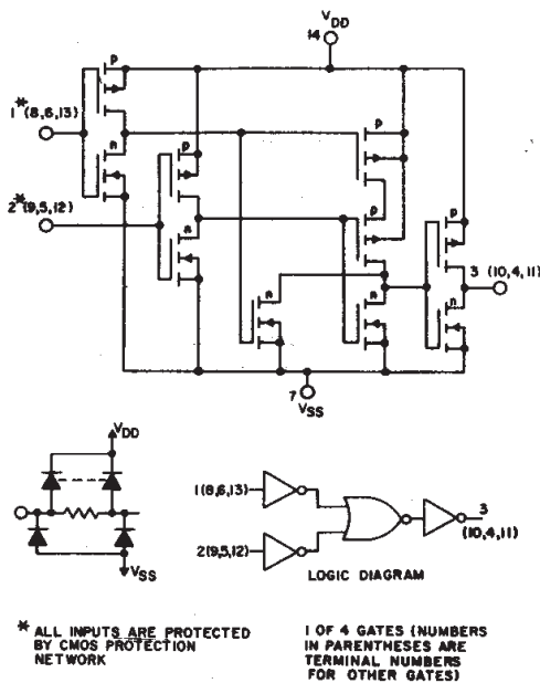
Fig. 7 — Schematic and logic diagrams for CD4011B.
