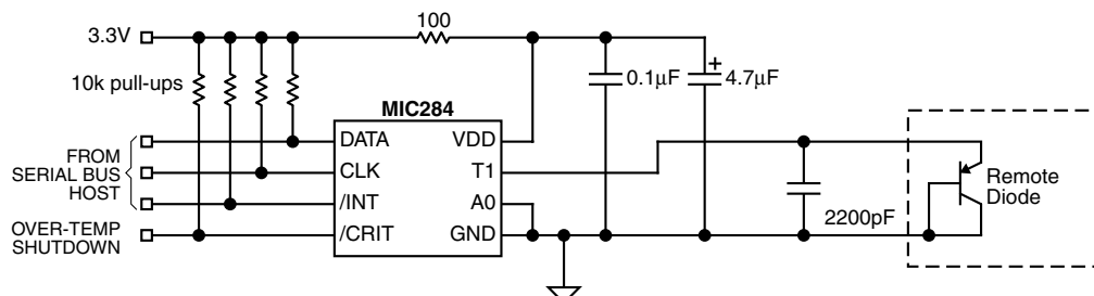
Figure 7. V_{DD} Decoupling for Very Noisy Supplies
