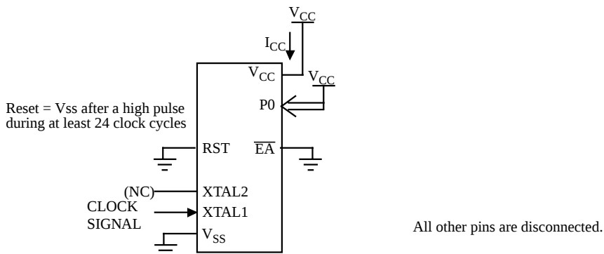
Figure 22. I_{CC} Test Condition, Idle Mode
