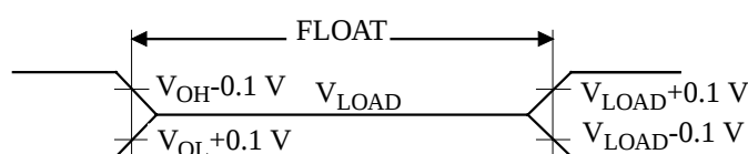
Figure 32. Float Waveforms
