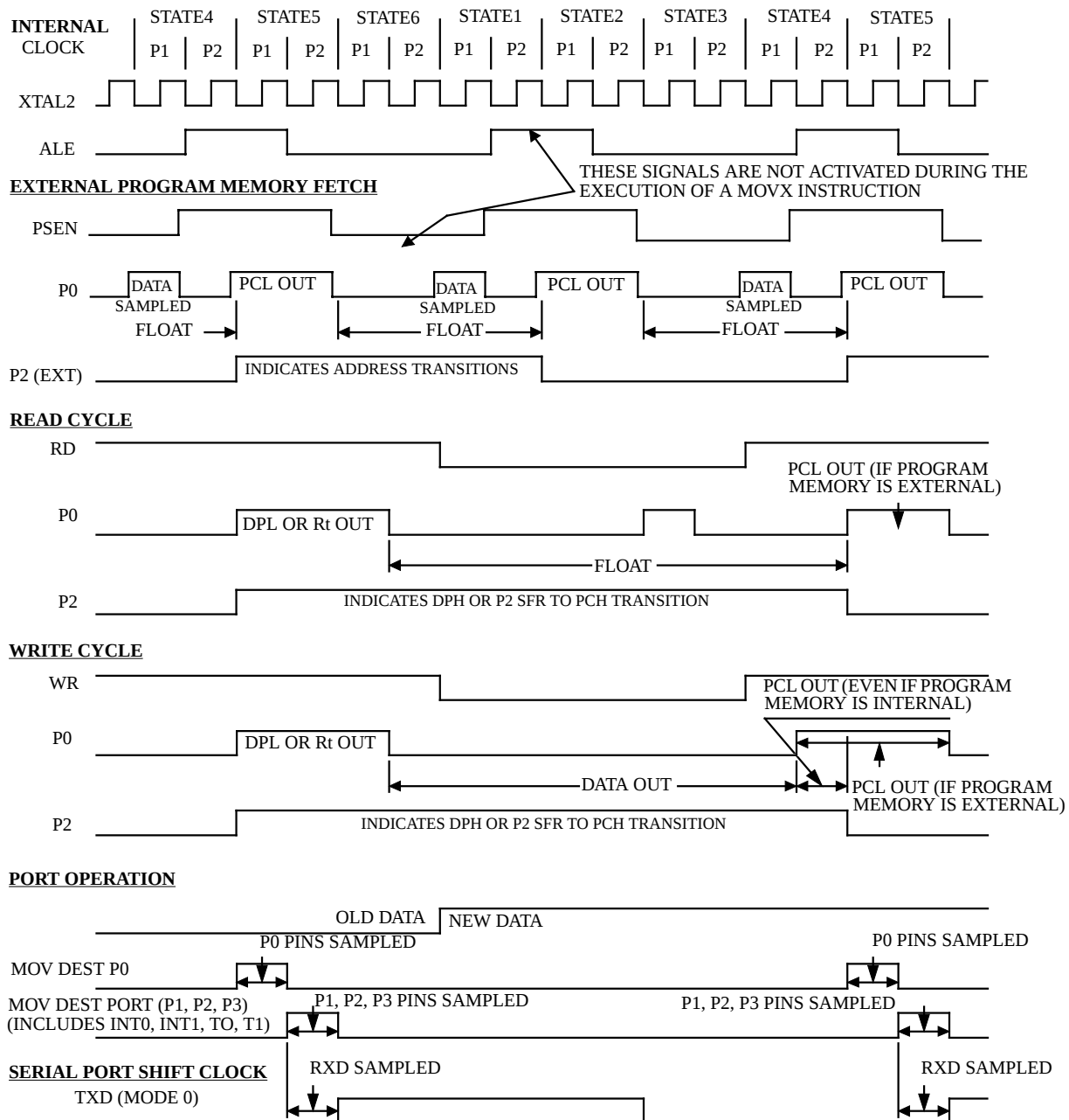
Figure 33. Clock Waveforms
