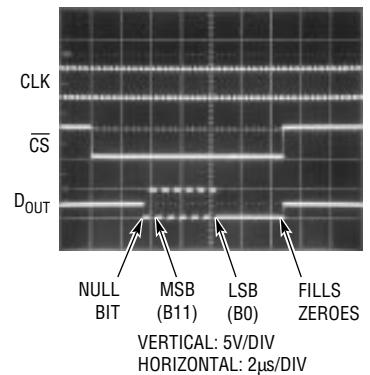
Figure 24. Scope Trace of the LTC1294/6 “Quick Look” Circuit Showing A/D Output 1010101010 (AA HEX )
