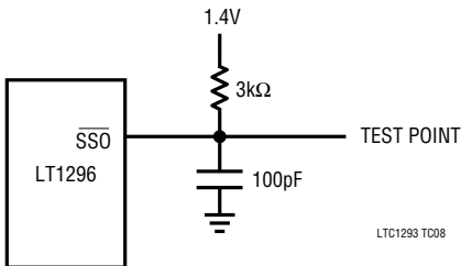
Load Circuit for t_{enSS0} and t_{disSS0}
