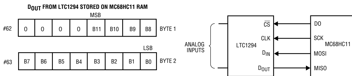
Hardware and Software Interface to Motorola MC68HC11
