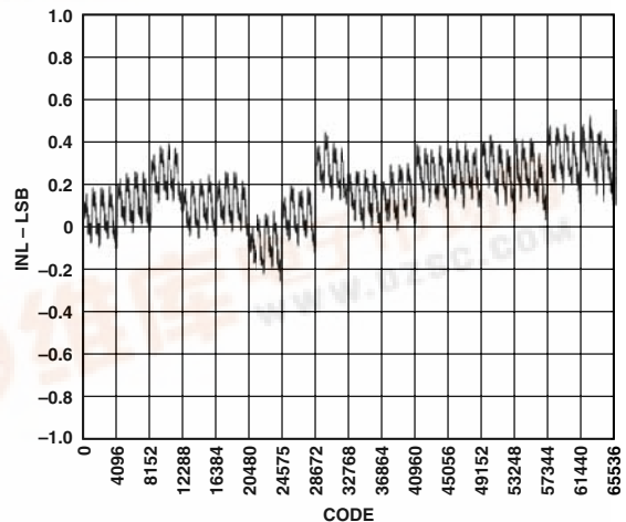
Figure 1. Integral Nonlinearity Error
