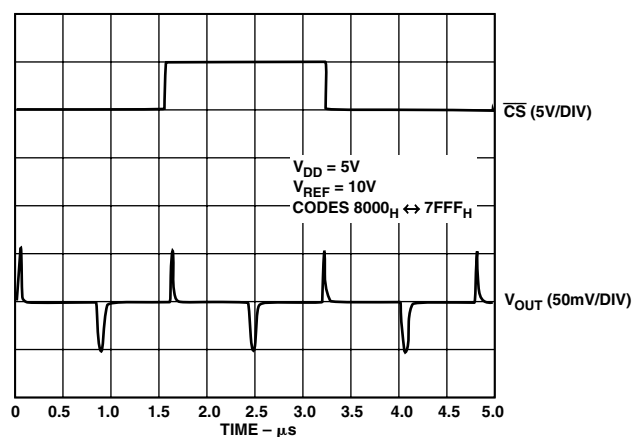
TPC 11. Midscale Transition and Digital Feedthrough
