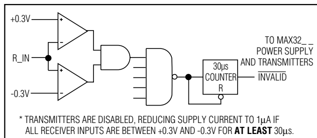
Figure 3a. MAX3221/MAX3223/MAX3243 Entering 1 \mu A Supply Mode via AutoShutdown
