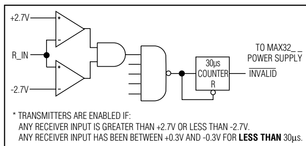
Figure 3b. MAX3221/MAX3223/MAX3243 with Transmitters Enabled Using AutoShutdown
