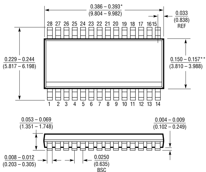
GN Package 28-Lead Plastic SSOP (Narrow .150 Inch) (Reference LTC DWG # 05-08-1641)
