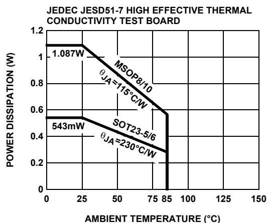
FIGURE 45. PACKAGE POWER DISSIPATION vs AMBIENT TEMPERATURE
