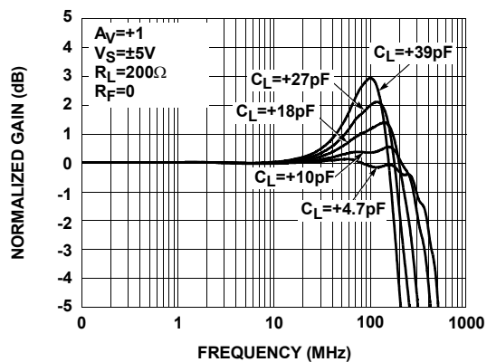
FIGURE 25. GAIN vs FREQUENCY FOR VARIOUS C_L
