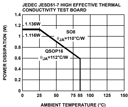
FIGURE 46. PACKAGE POWER DISSIPATION vs AMBIENT TEMPERATURE
