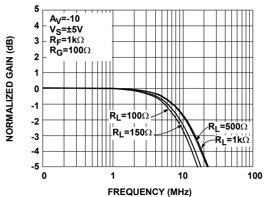
FIGURE 23. GAIN vs FREQUENCY FOR VARIOUS R_L
