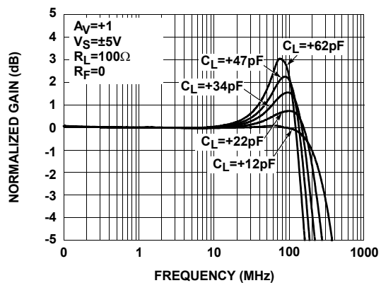
FIGURE 26. GAIN vs FREQUENCY FOR VARIOUS C_L
