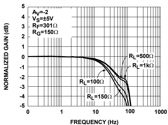
FIGURE 22. GAIN vs FREQUENCY FOR VARIOUS R_L
