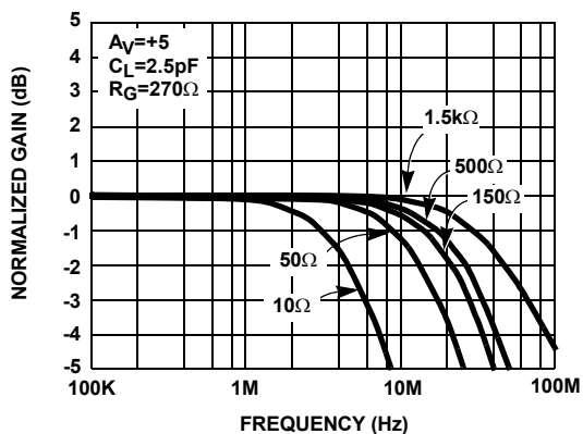
FIGURE 4. GAIN vs FREQUENCY FOR VARIOUS R_L
