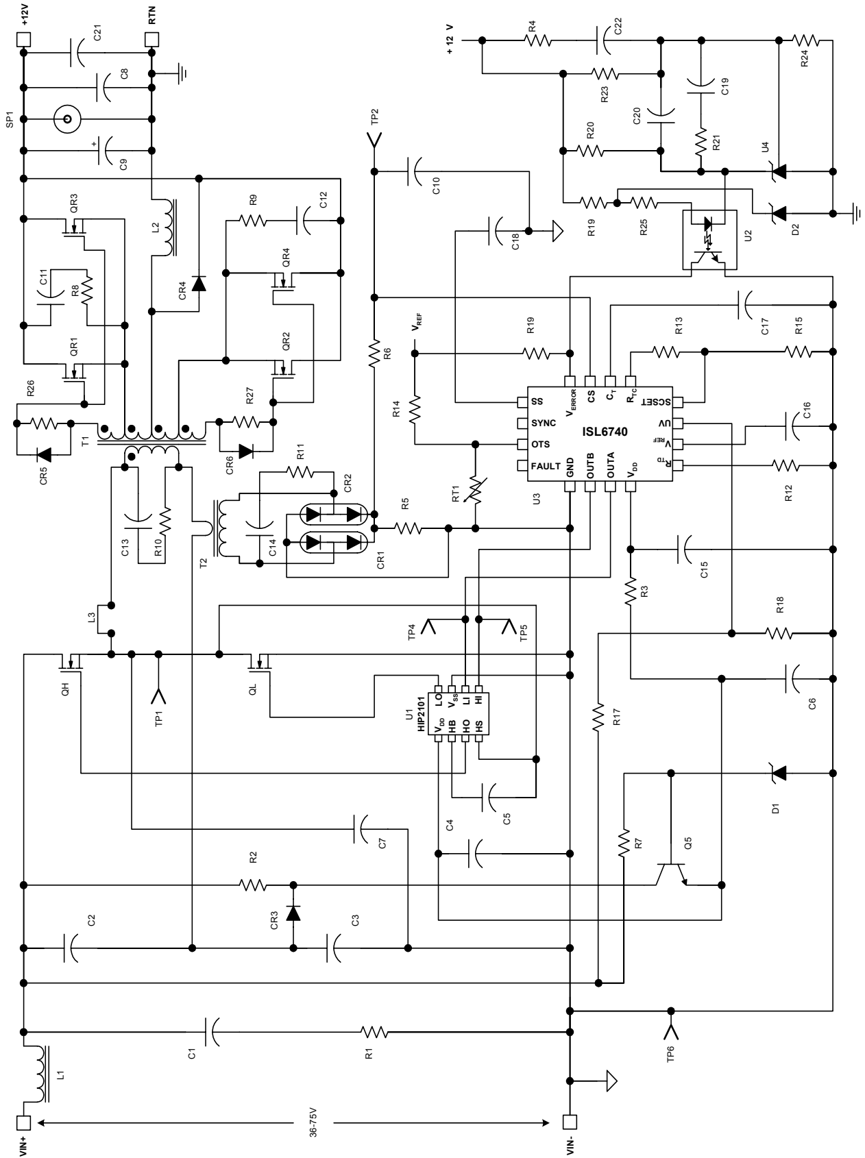
Typical Application (ISL6740) - 36 to 75 V Input, Regulated 12V @ 8A Output (ISL6740EVAL2)
