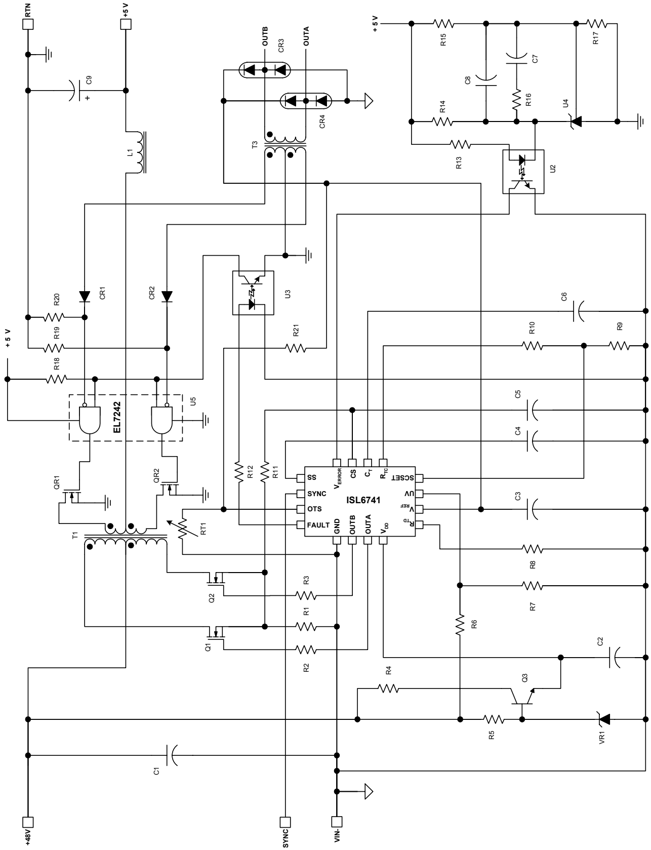
Typical Application (ISL6741) - 48 to 5 Volt Push-Pull DC-DC Converter
